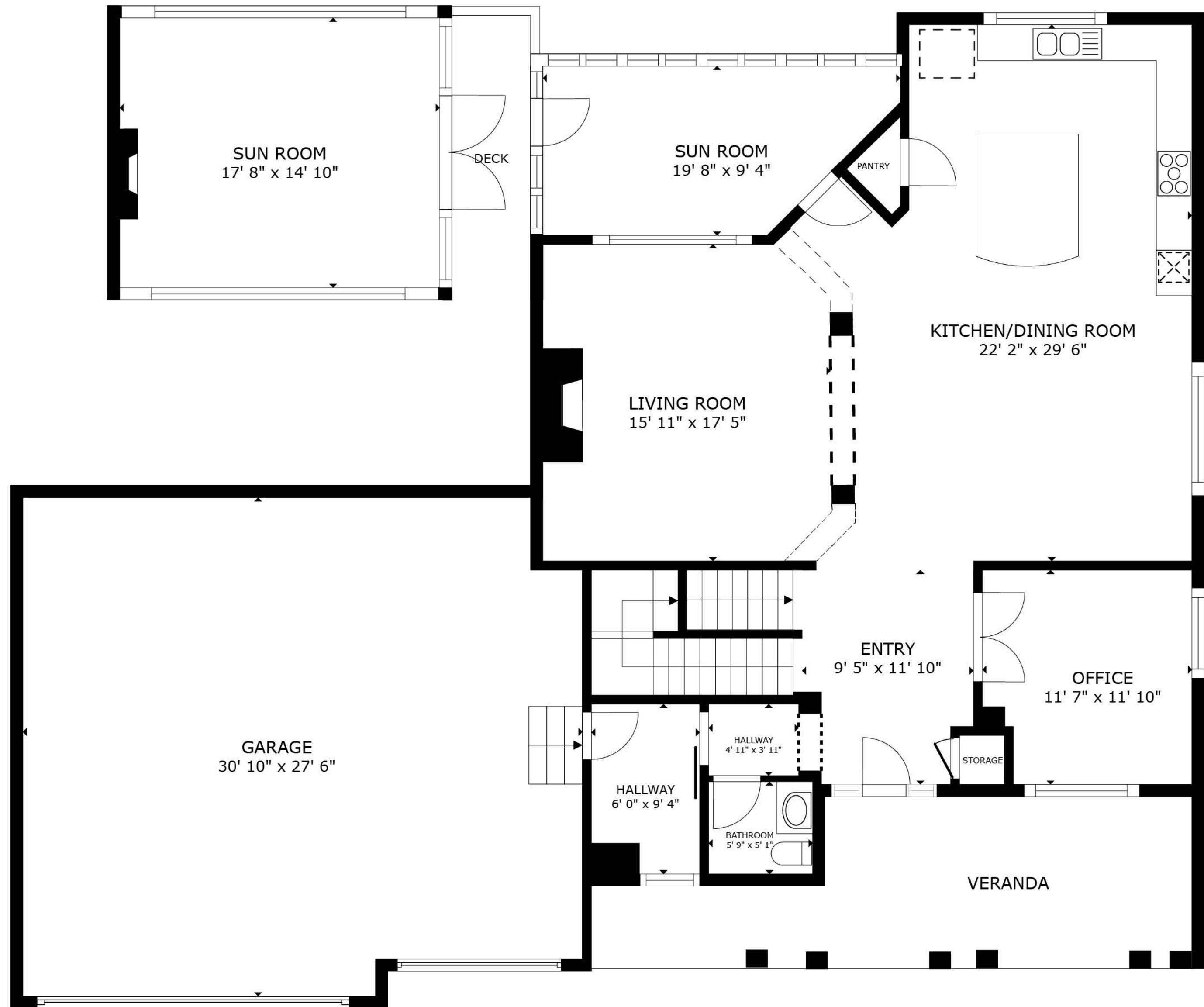
FLOOR 2
